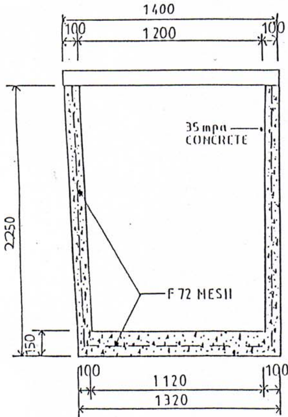
SECTION
